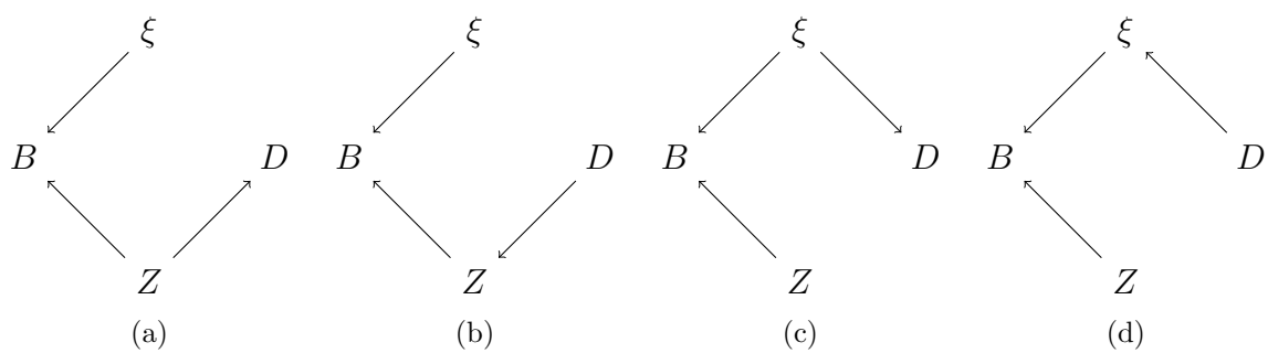
Figure 2: Causal DAGs for the four instances given in Section 3.2.
